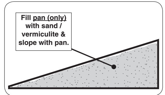
Fig. 21-2 Sand/vermiculite detail
