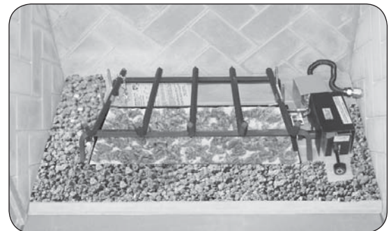
Fig. 22-3 Place grate
